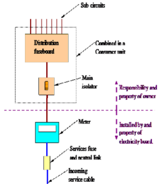
SCHMATIC DIAGRAM OF DOMESTIC INCOMING ELECTRICAL SERVICE
