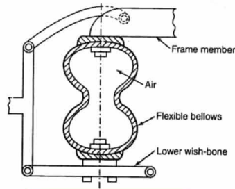
Figure Bellow type air spring
