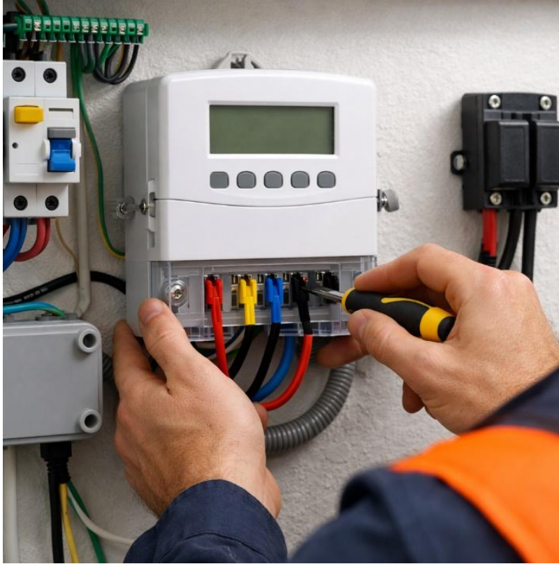
Installation of energy meter
