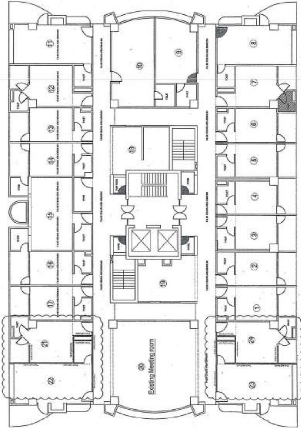
LEVEL 15 EXISTING FLOOR PLAN (5" BRICK WALL DEMOLISH ) AT-71-72 ELEPHANT ROAD, DHAKA
