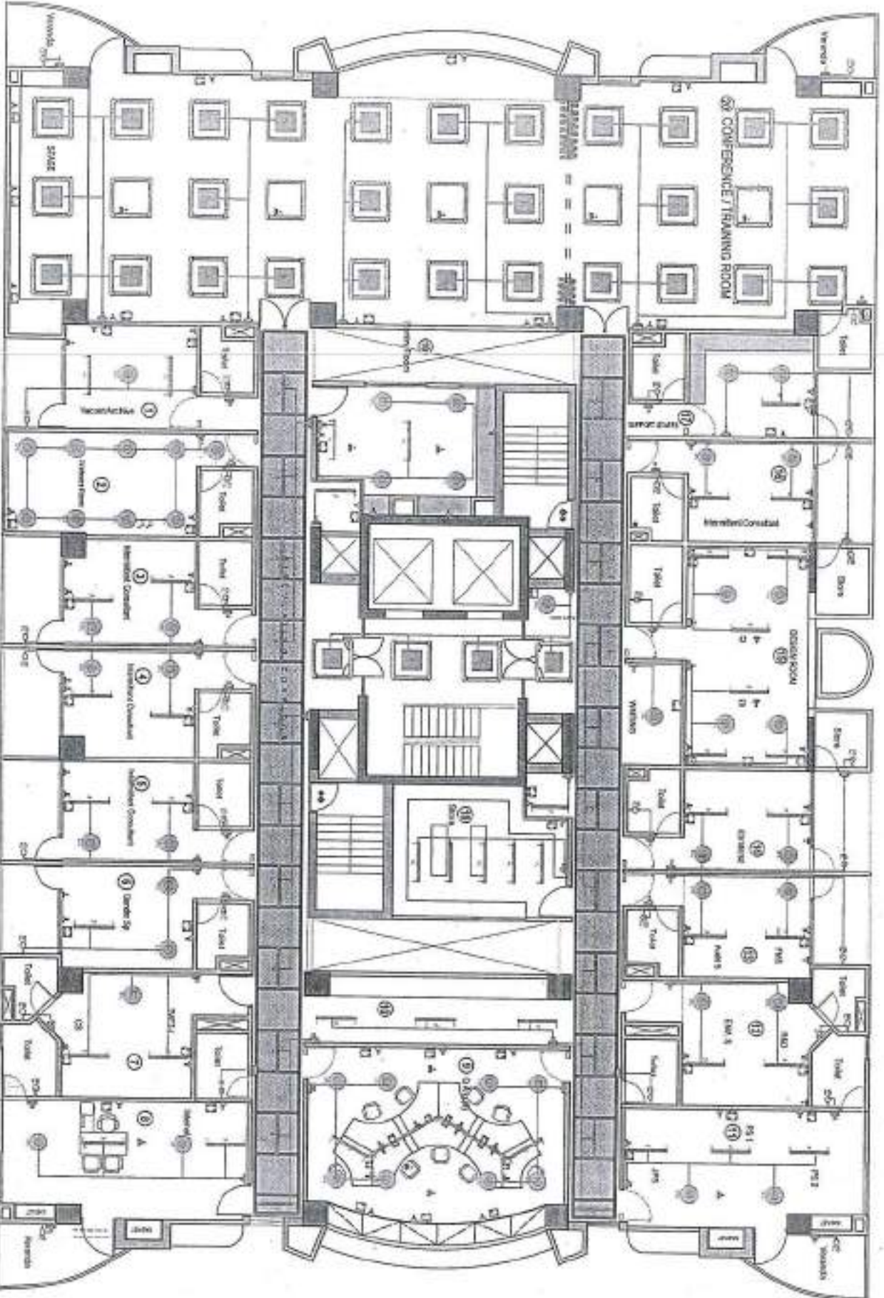
LEVEL 14 PROPOSED ELECTRIC LAY-OUT PLAN FOR SICIP AT-71-72 ELEPHANT ROAD, DHAKA
